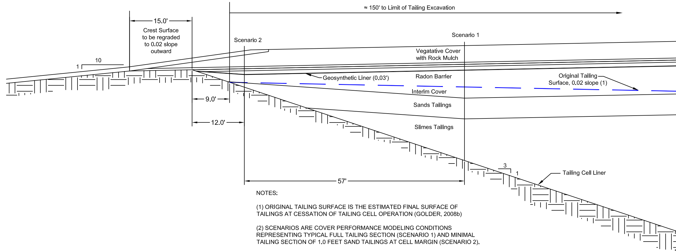
TYPICAL SECTION FOR TAILING REGRADING AND COVER AT MARGIN OF CELL
