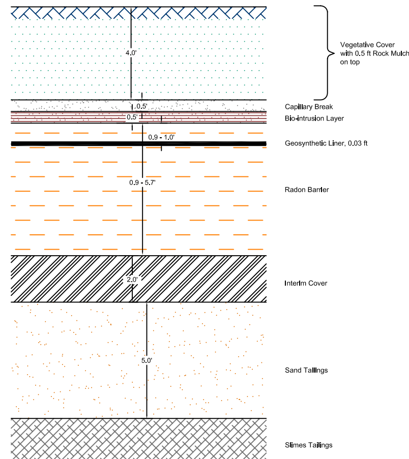
TYPICAL SECTION FOR TAILING CELL COVER
