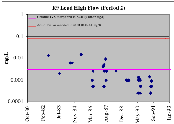
Figure A-3 (cont'd). Upper Arkansas River Dissolved Lead Concentrations in Period 2 (1981-1992), as reported in SCR 2002
