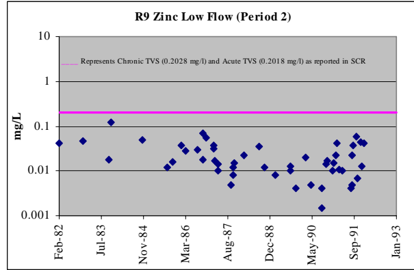
Figure A-4 (cont'd). Upper Arkansas River Dissolved Zinc Concentrations in Period 2 (1981-1992), as reported in SCR 2002
