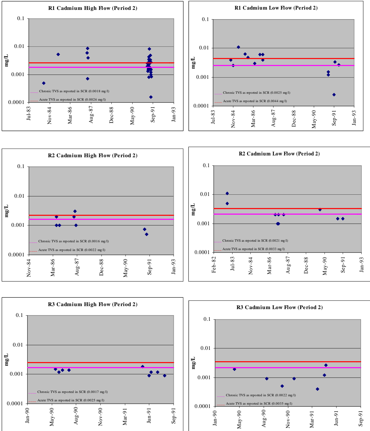
Figure A-1. Upper Arkansas River Dissolved Cadmium Concentrations in Period 2 (1981-1992), as reported in SCR 2002
