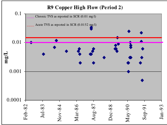
Figure A-2 (cont'd). Upper Arkansas River Dissolved Copper Concentrations in Period 2 (1981-1992), as reported in SCR 2002
