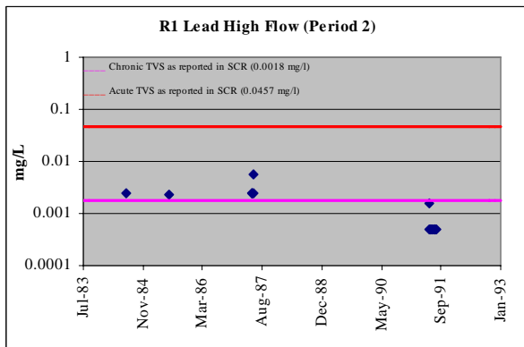
Figure A-3. Upper Arkansas River Dissolved Lead Concentrations in Period 2 (1981-1992), as reported in SCR 2002
