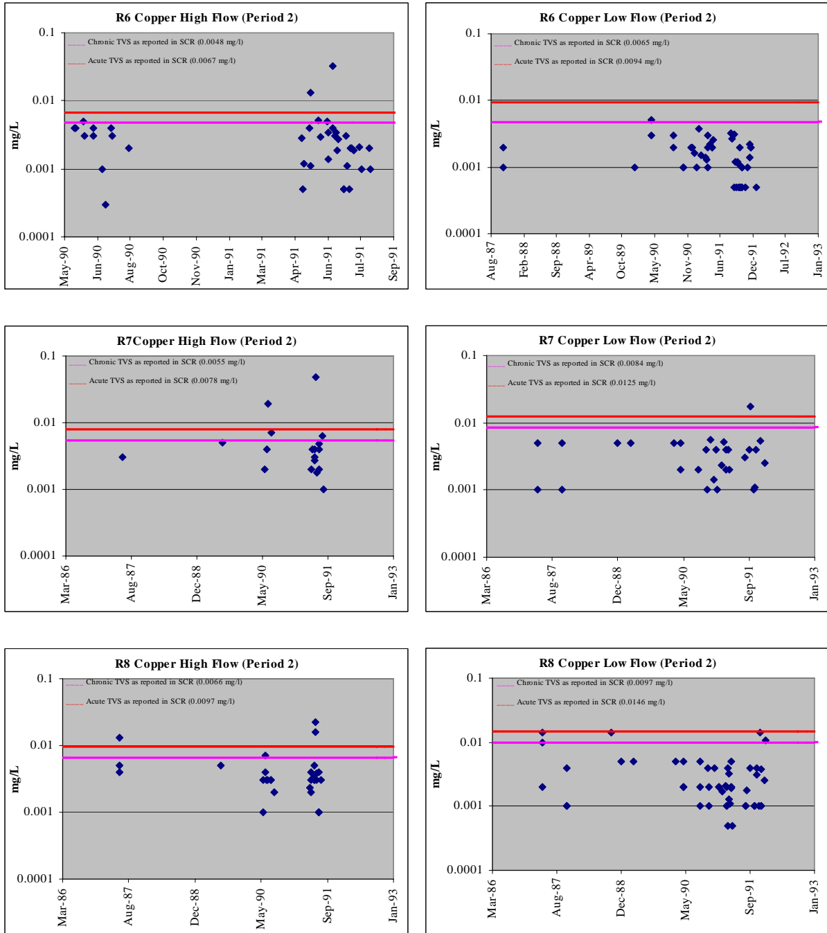
Figure A-2 (cont'd). Upper Arkansas River Dissolved Copper Concentrations in Period 2 (1981-1992), as reported in SCR 2002
