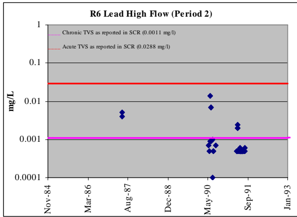
Figure A-3 (cont'd). Upper Arkansas River Dissolved Lead Concentrations in Period 2 (1981-1992), as reported in SCR 2002
