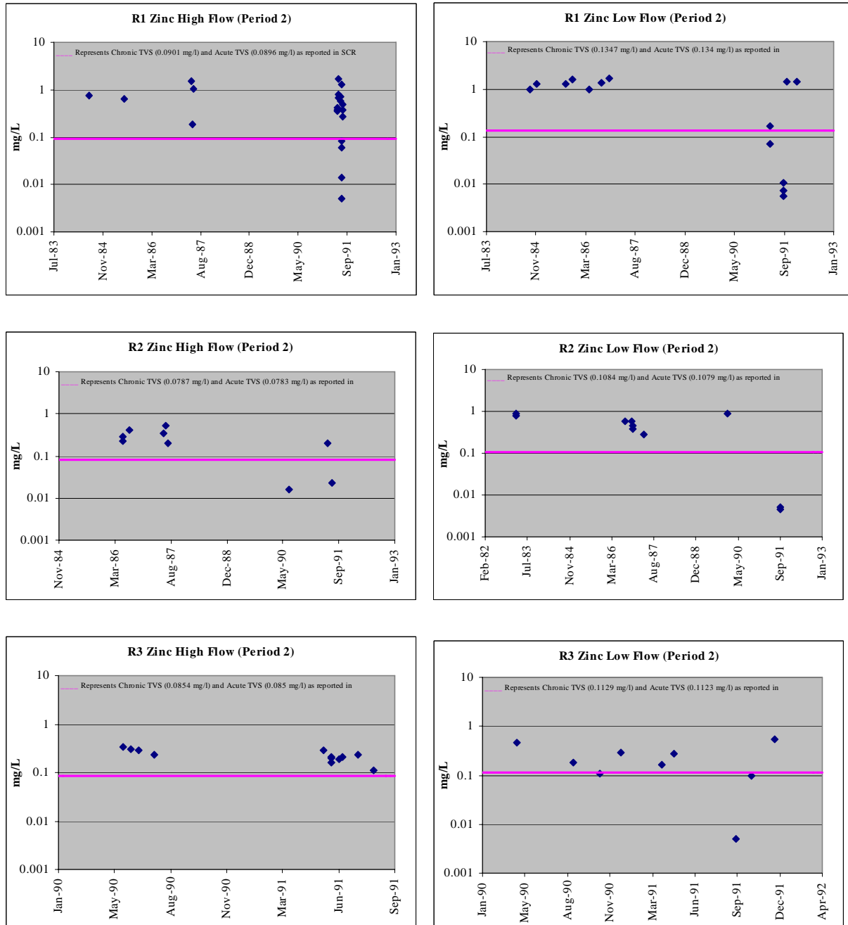
Figure A-4. Upper Arkansas River Dissolved Zinc Concentrations in Period 2 (1981-1992), as reported in SCR 2002
