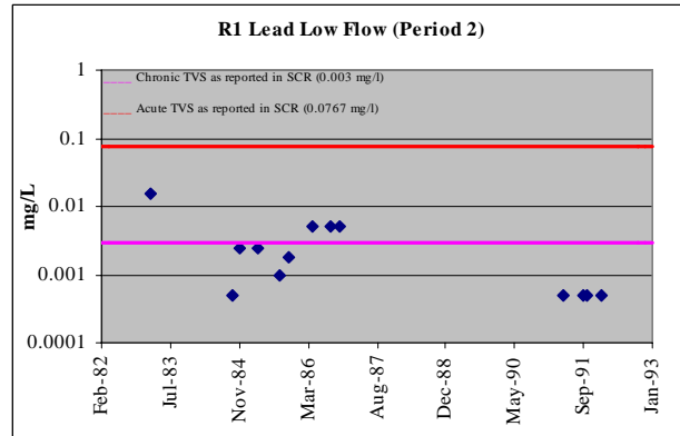
Figure A-3. Upper Arkansas River Dissolved Lead Concentrations in Period 2 (1981-1992), as reported in SCR 2002
