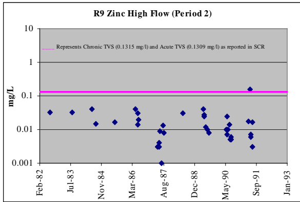
Figure A-4 (cont'd). Upper Arkansas River Dissolved Zinc Concentrations in Period 2 (1981-1992), as reported in SCR 2002
