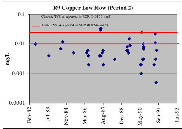
Figure A-2 (cont'd). Upper Arkansas River Dissolved Copper Concentrations in Period 2 (1981-1992), as reported in SCR 2002
