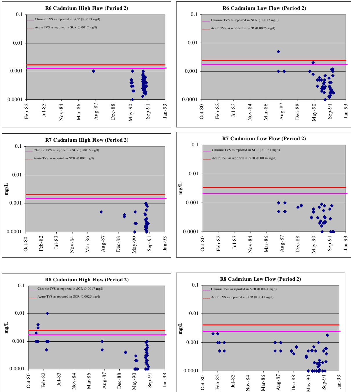
Figure A-1 (cont'd). Upper Arkansas River Dissolved Cadmium Concentrations in Period 2 (1981-1992), as reported in SCR 2002
